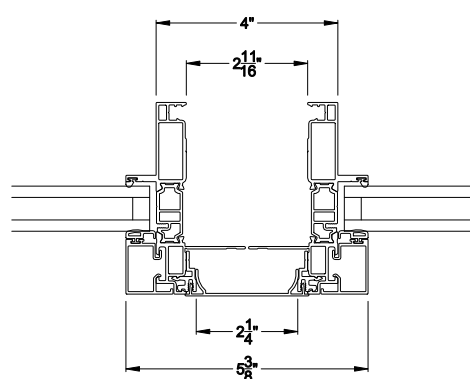
VUE COLLECTION SPREAD MULLS 2 1/4" mull cover
