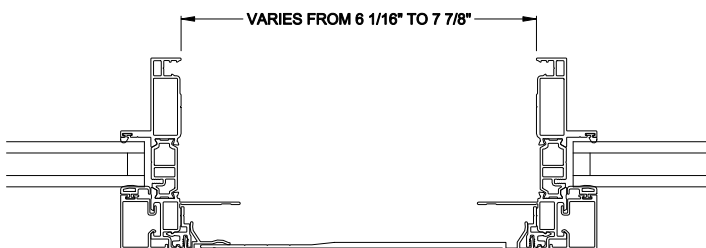
VUE COLLECTION SPREAD MULLS 2 Piece mull cover - Mid
