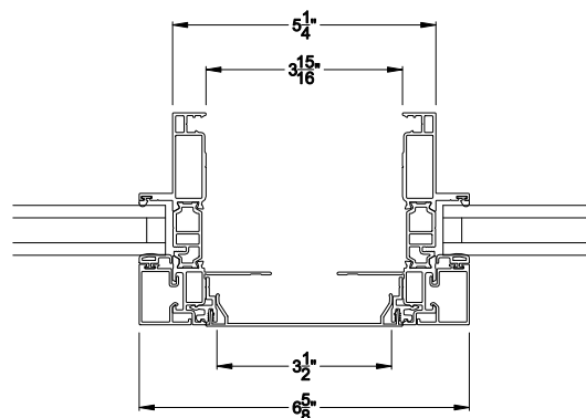
VUE COLLECTION SPREAD MULLS 3 1/2" mull cover
