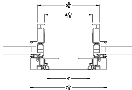
VUE COLLECTION SPREAD MULLS 4" mull cover
