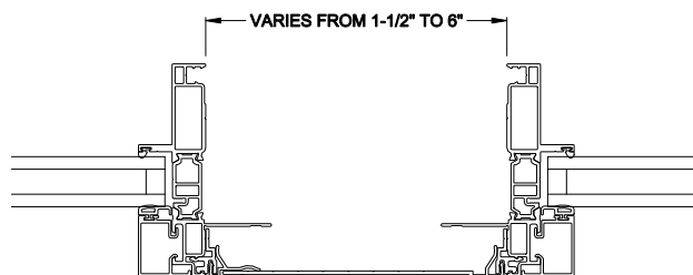
VUE COLLECTION SPREAD MULLS 2 Piece mull cover
