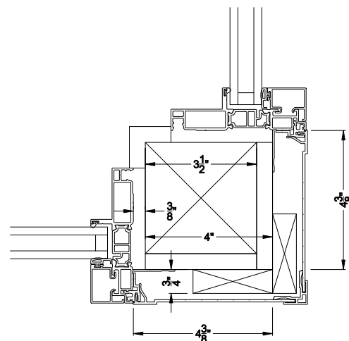
VUE COLLECTION 90 DEGREE CORNER MULL 3 Piece mull cover around Field Framing
