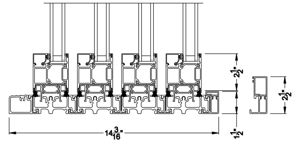
VUE COLLECTION MULTI-SLIDE WINDOW (4701) Vertical Section - with Sill Riser - 4 or Bi-parting 8 Panel Window
