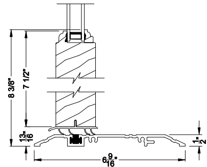
PREMIUM WOOD OUTSWING DOOR (6610) Vertical Section - ADA Sill
