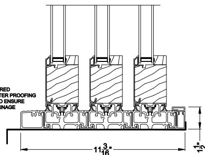
CONTEMPORARY 2-1/4" MULTI-SLIDE PATIO DOOR (8726) Vertical Section - With sill pan
