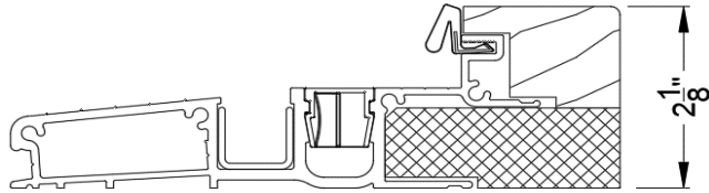
Standard Sill
