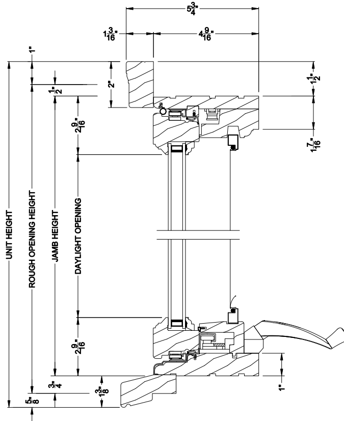
WEATHER SHIELD FRENCH CASEMENT WINDOW (6204) Vertical Section
