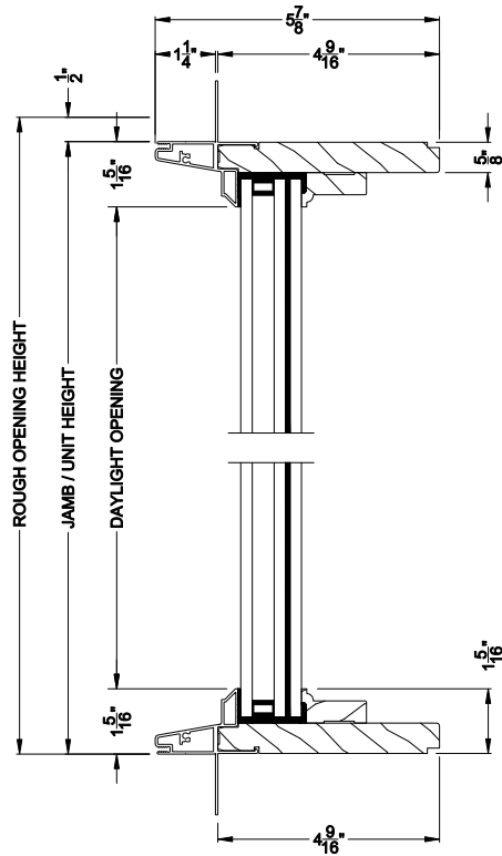
PREMIUM COASTAL IG DIRECT-SET (1311) Vertical Section - Slim Frame
