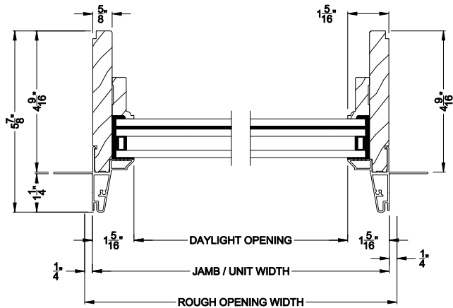
PREMIUM COASTAL IG DIRECT-SET (1311) Horizontal Section - Slim Frame
