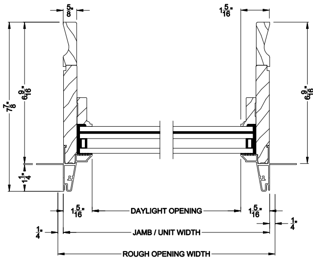
PREMIUM COASTAL IG DIRECT-SET (1311) Horizontal Section - Slim Frame
