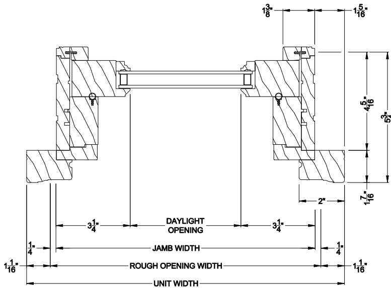
PREMIUM WOOD DOUBLE HUNG PICTURE (6122) Horizontal Section
