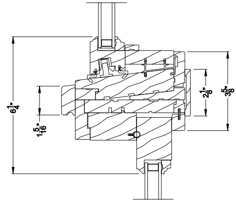
PREMIUM WOOD DOUBLE HUNG PICTURE Horizontal Stack Section - Transom Stack over Picture
