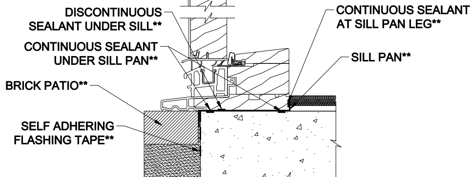
Vertical Section Detail - Standard Sill
