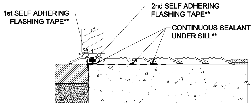
Vertical Section Detail - ADA Sill
