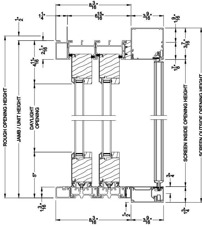
CONTEMPORARY 2-1/4" MULTI-SLIDE PATIO DOOR (8726) Vertical Section - Standard Sill - 2 or Bi-parting 4 Panel Door Shown with optional Center screen - recess mounted
