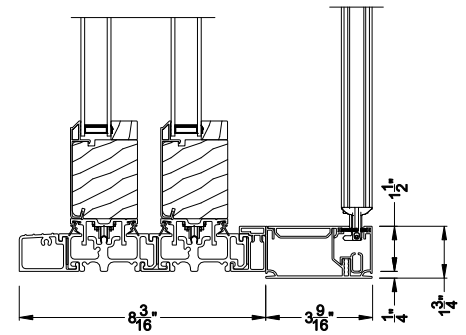
CONTEMPORARY 2-1/4" MULTI-SLIDE PATIO DOOR (8726) Vertical Section - with Sill Riser - 2 or Bi-parting 4 Panel Door Shown with optional Center screen - recess mounted
