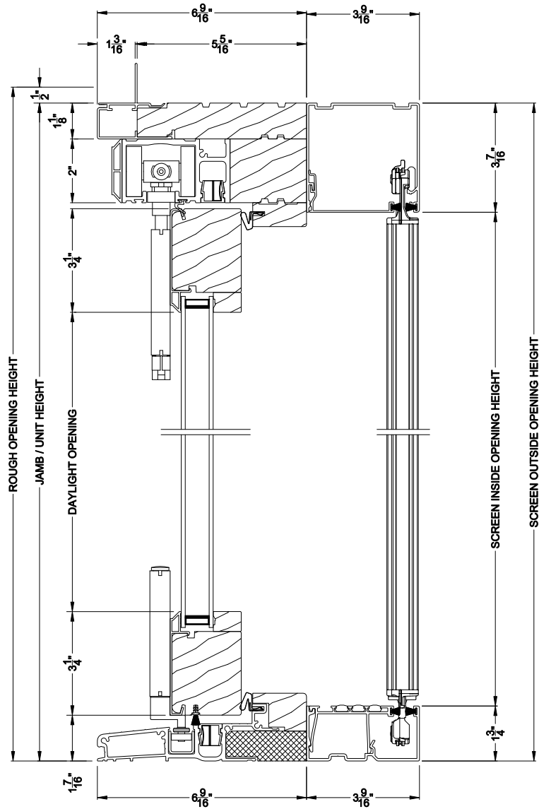
CONTEMPORARY BI-FOLD DOOR (8623) Vertical Section - Standard Sill - 3-1/4" Bottom Rail Shown with optional Center screen
