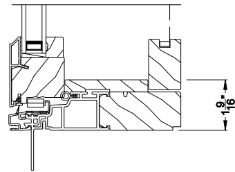
Shown with Optional Wood Hinged Screen CONTEMPORARY CASEMENT WINDOW (8220) Vertical Section - Manual Push Out - Low Profile Sill
