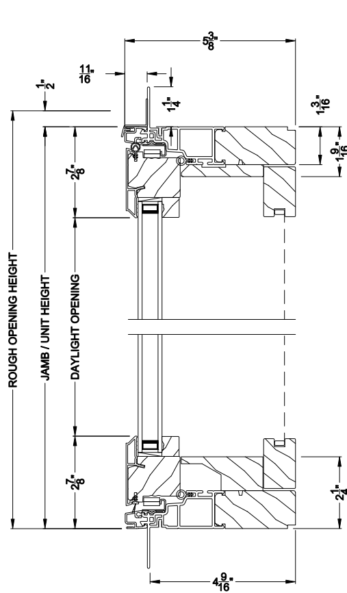
Shown with Optional Wood Hinged Screen CONTEMPORARY CASEMENT WINDOW (8220) Vertical Section - Flush Frame - Manual Push Out
