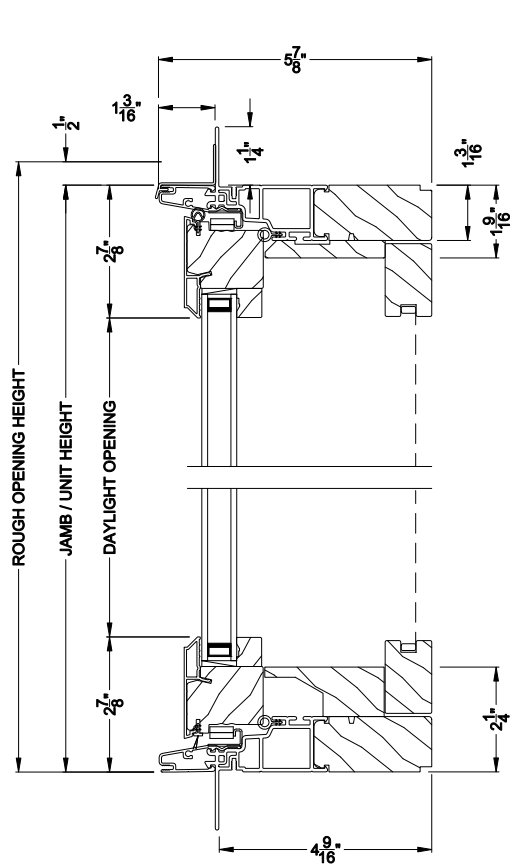
Shown with Optional Wood Hinged Screen CONTEMPORARY CASEMENT WINDOW (8217) Vertical Section - Shadow-Line Frame - Manual Push Out
