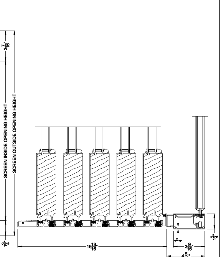
PREMIUM 2-1/4" MULTI-SLIDE PATIO DOOR (8721)
