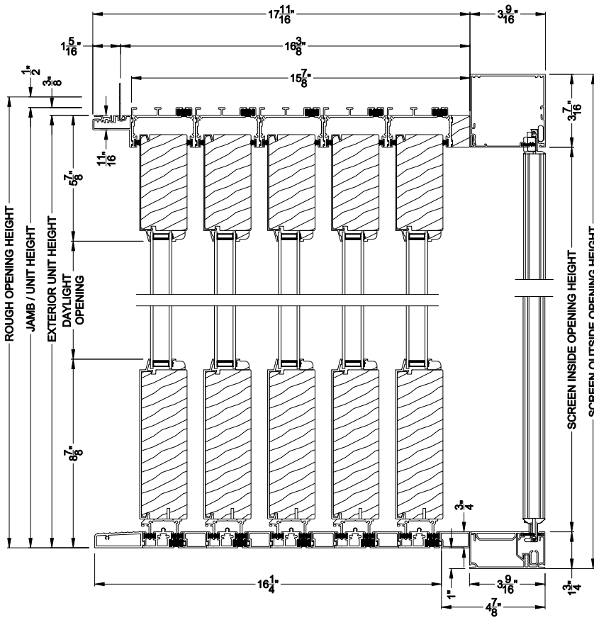
PREMIUM 2-1/4" MULTI-SLIDE PATIO DOOR (8721)
