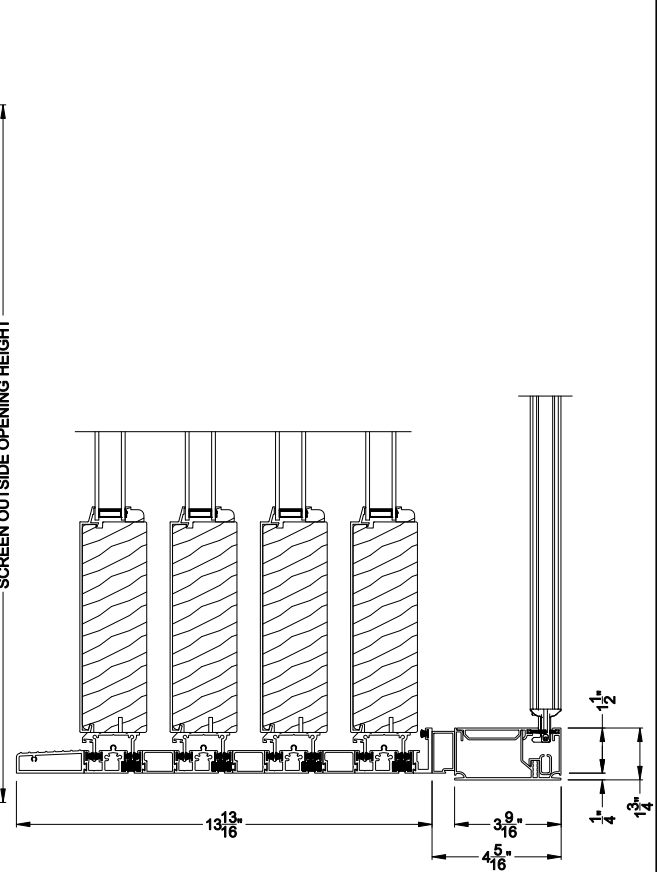
PREMIUM 2-1/4" MULTI-SLIDE PATIO DOOR (8721)
