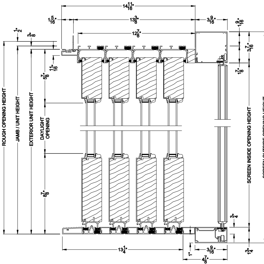
PREMIUM 2-1/4" MULTI-SLIDE PATIO DOOR (8721)
