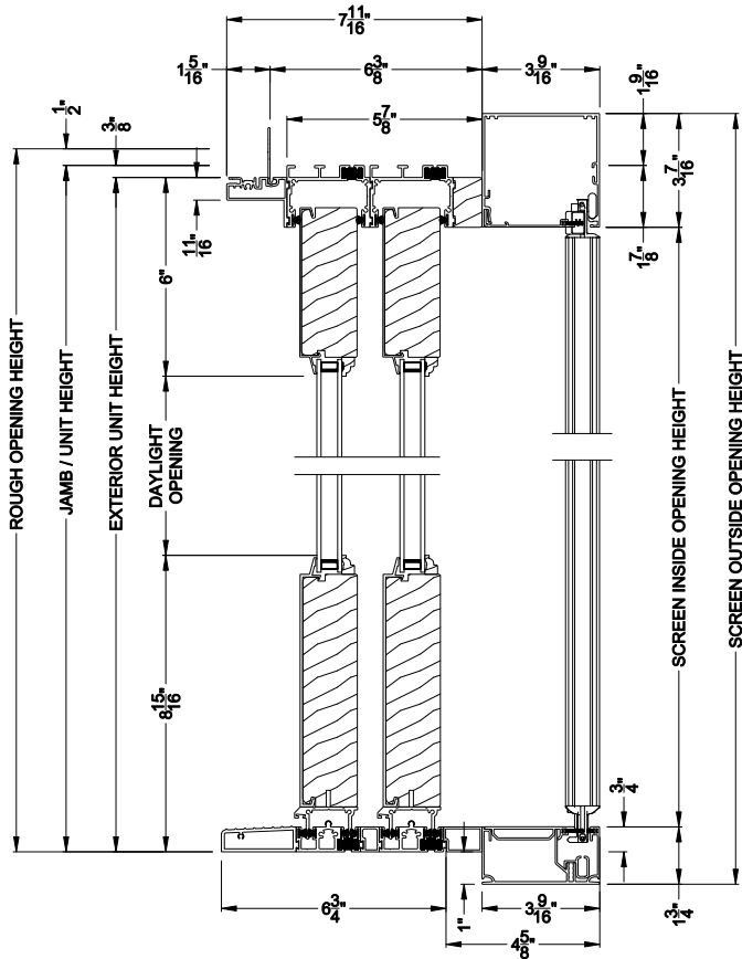
PREMIUM 1-3/4" MULTI-SLIDE PATIO DOOR (8719) Vertical Section - Standard Sill - 2 or Bi-parting 4 Panel Door Shown with optional Center screen - recess mounted
