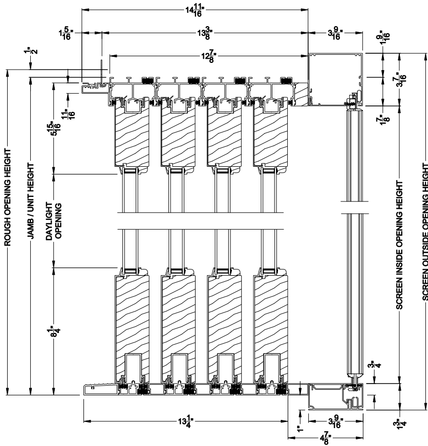
PREMIUM LIFT & SLIDE PATIO DOOR (8716) Vertical Section - Standard Sill - 4 or Bi-parting 8 Panel Door Shown with optional Center screen - flush mounted
