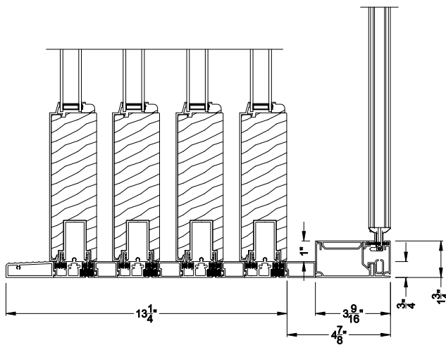
PREMIUM LIFT & SLIDE PATIO DOOR (8716) Vertical Section - Standard Sill - 4 or Bi-parting 8 Panel Door Shown with optional Center screen - flush mounted
