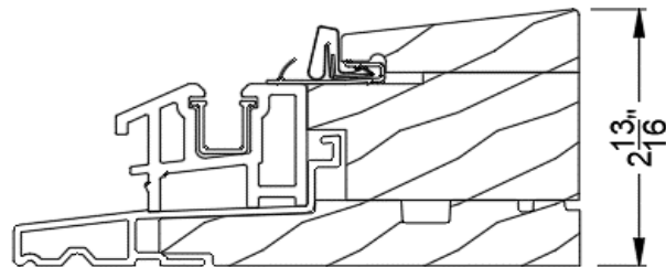
Standard Sill
