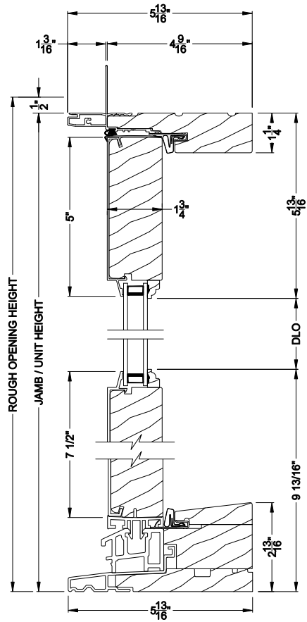
PREMIUM OUTSWING SIDELITE (8610) Vertical Section
