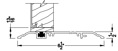
PREMIUM OUTSWING SIDELITE (8610) Vertical Section - ADA Sill
