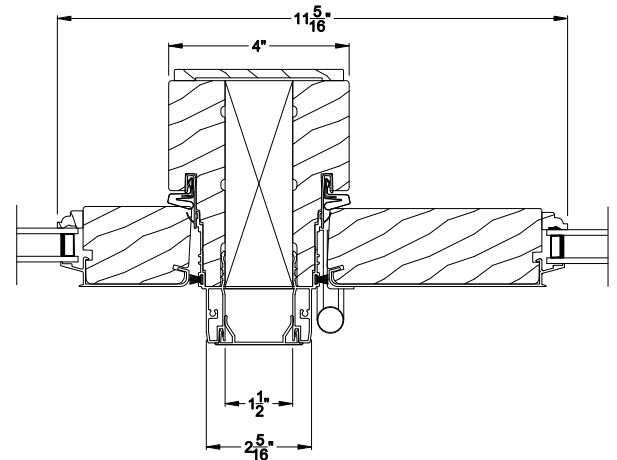
PREMIUM OUTSWING DOOR (8610) Vertical Mull Section - Sidelite / Oper
