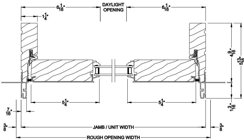
PREMIUM OUTSWING DOOR (8610) Horizontal Section - Stationary Single Door
