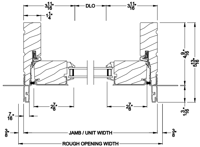
PREMIUM OUTSWING SIDELITE (8610) Horizontal Section
