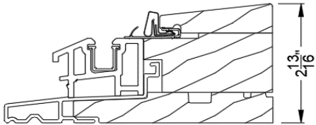
Standard Sill
