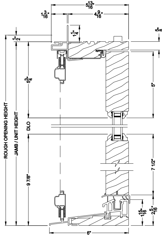
ASPIRE CENTER HINGE DOOR (7502) Vertical Section
