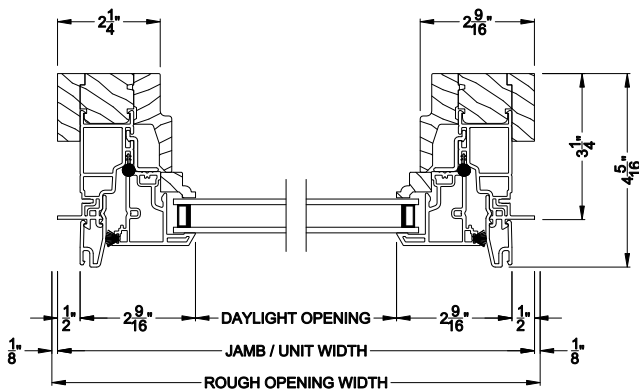
ASPIRE POCKET CASEMENT PICTURE WINDOW (7206) Horizontal Section
